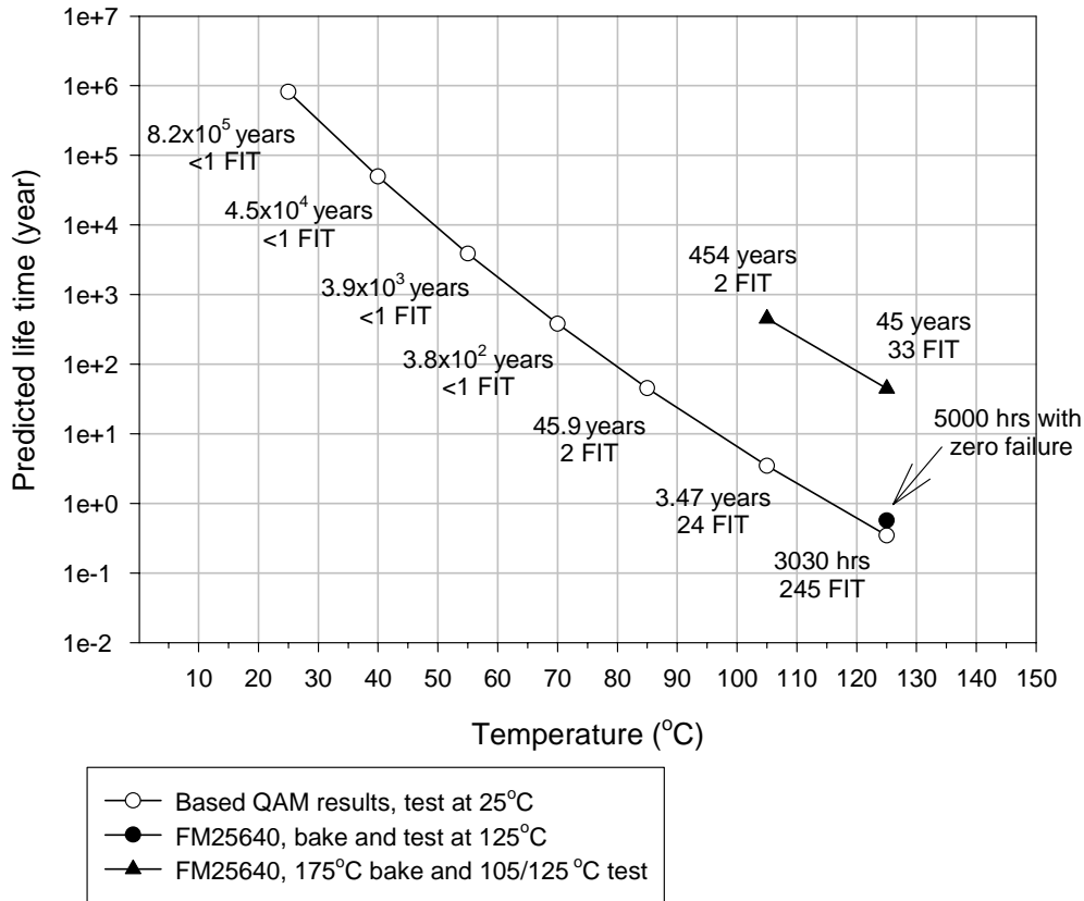
Figure 1. 5V 2T2C and 5V 1T1C Data Retention Prediction based on E A = 1.5 eV (60% C.I.)
