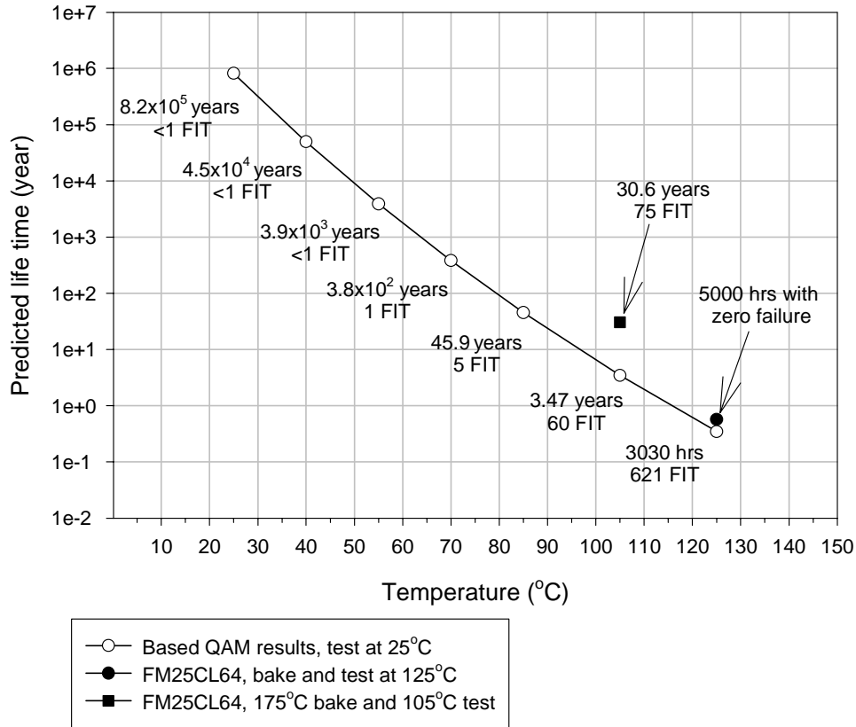
Figure 2. 3V 2T2C Data Retention Prediction based on E_A = 1.5 \text{ eV} (60% C.I.)
